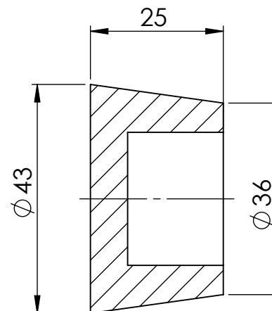
SECTION Y-Y
