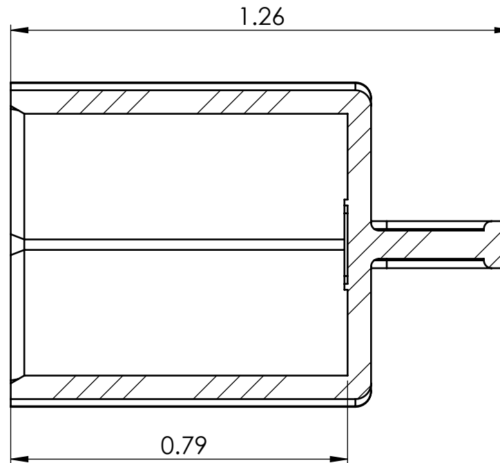
SECTION Y-Y
