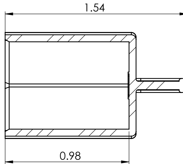
SECTION Y-Y
