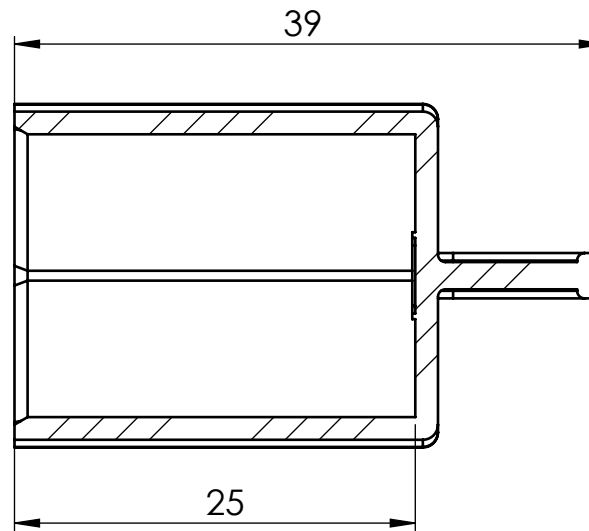
SECTION Y-Y
