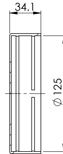
SECTION Y-Y
