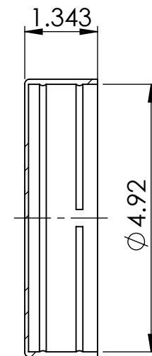
SECTION Y-Y
