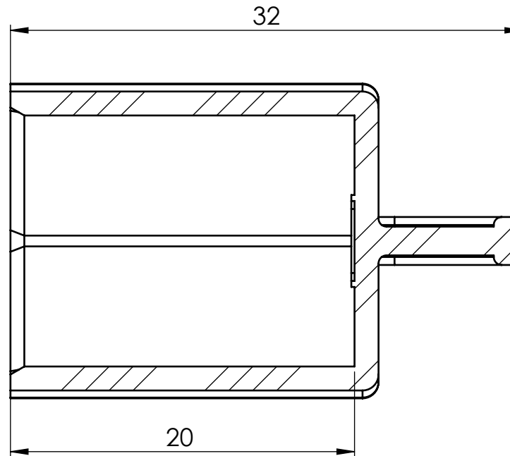
SECTION Y-Y
