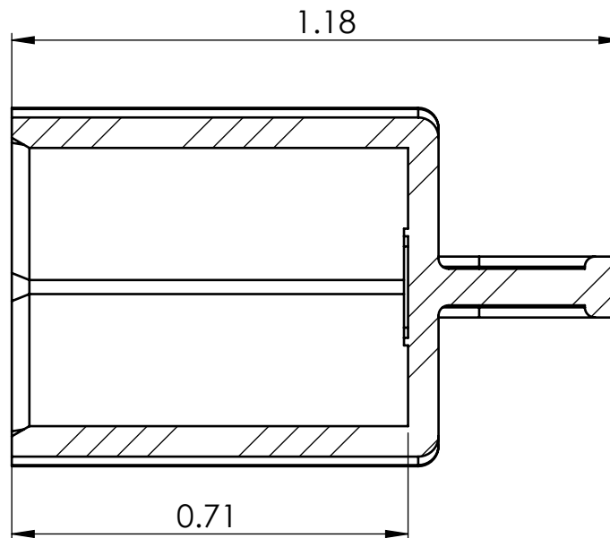
SECTION Y-Y
