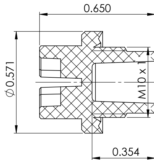
SECTION Y-Y
