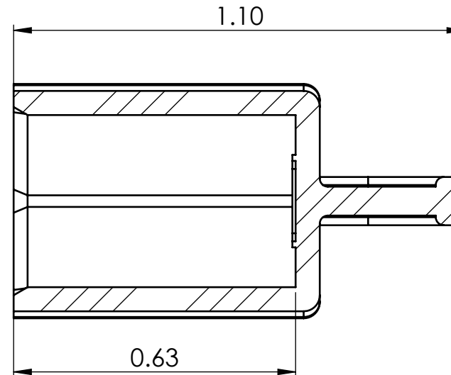
SECTION Y-Y
