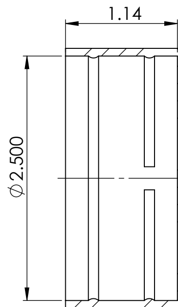
SECTION Y-Y
