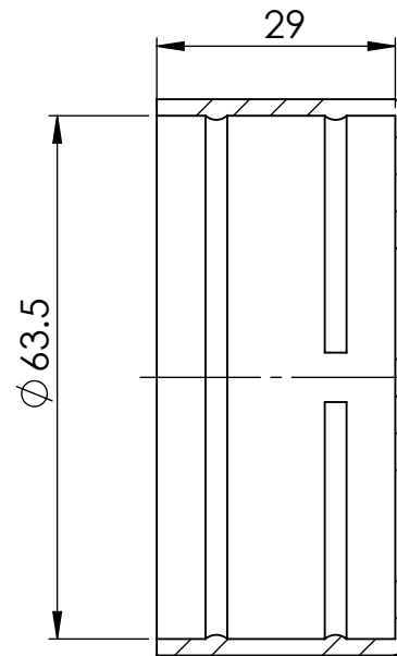
SECTION Y-Y
