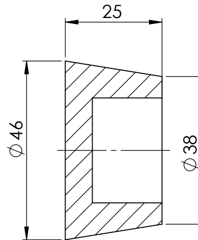
SECTION Y-Y
