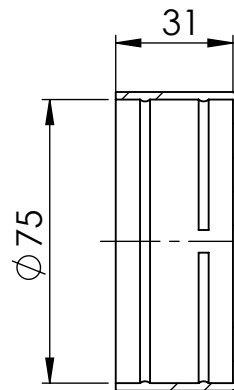
SECTION Y-Y
