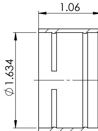
SECTION Y-Y
