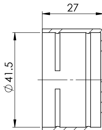
SECTION Y-Y
