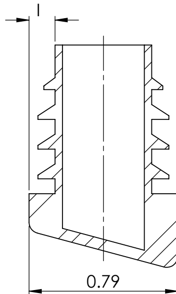
SECTION X-X
