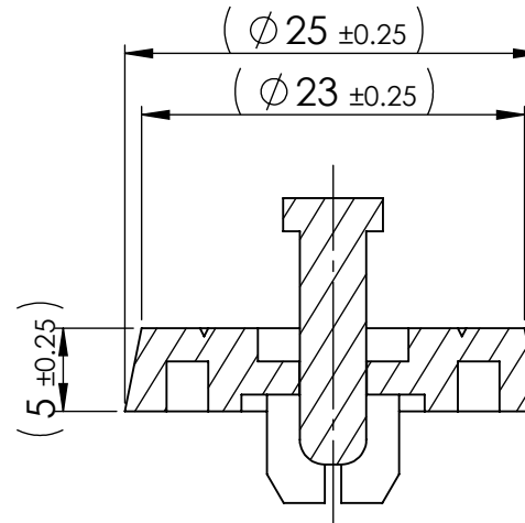
SECTION Y-Y
