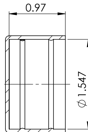
SECTION Y-Y
