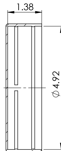
SECTION Y-Y
