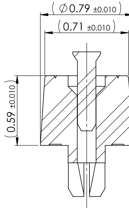
SECTION Y-Y
