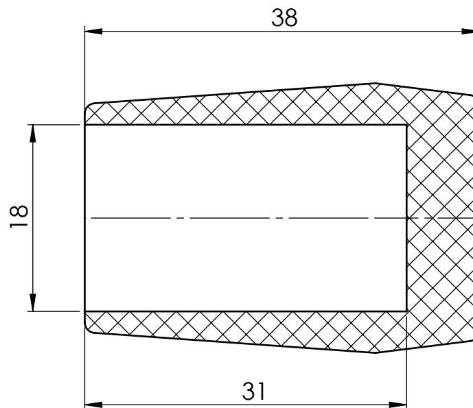
SECTION Y-Y
