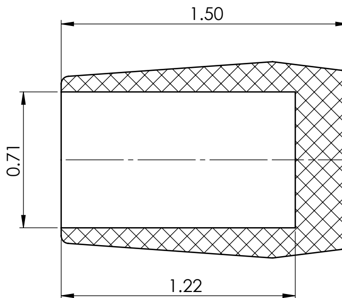
SECTION Y-Y
