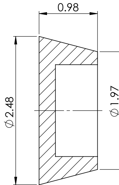
SECTION Y-Y
