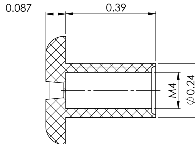
SECTION Y-Y
