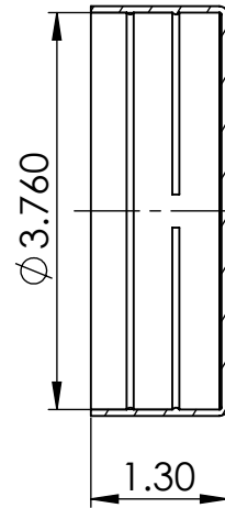
SECTION Y-Y
