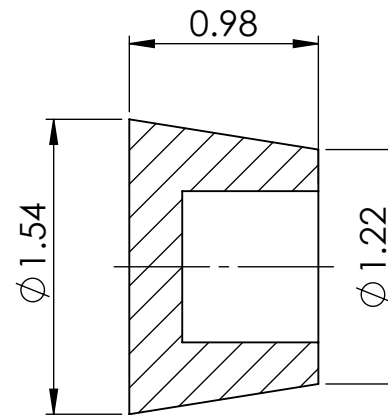
SECTION Y-Y
