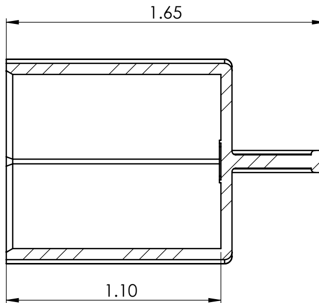
SECTION Y-Y
