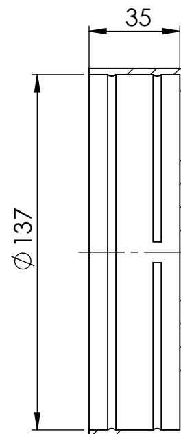
SECTION Y-Y
