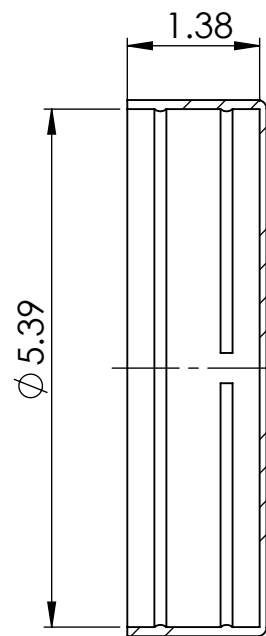
SECTION Y-Y
