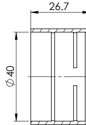
SECTION Y-Y
