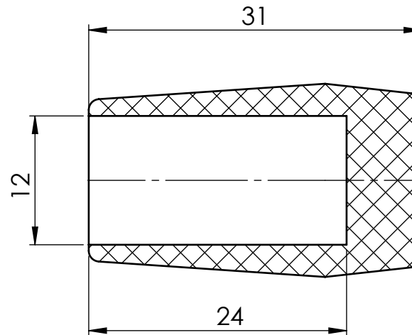
SECTION Y-Y
