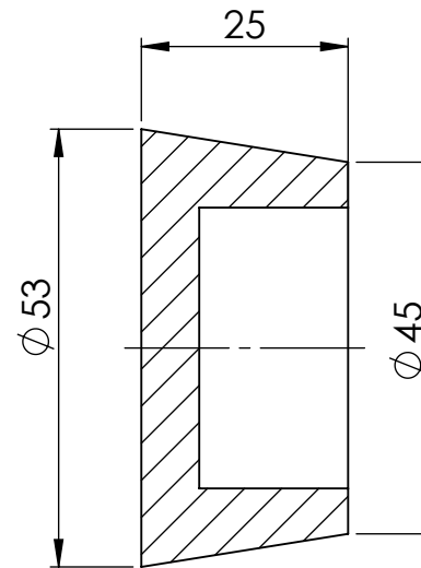
SECTION Y-Y
