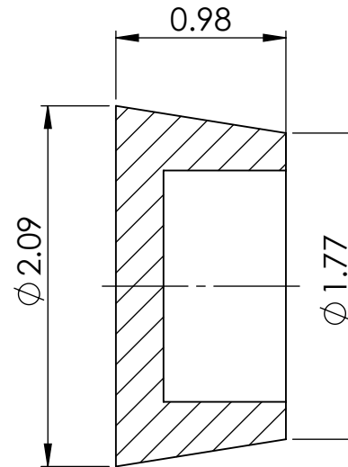
SECTION Y-Y
