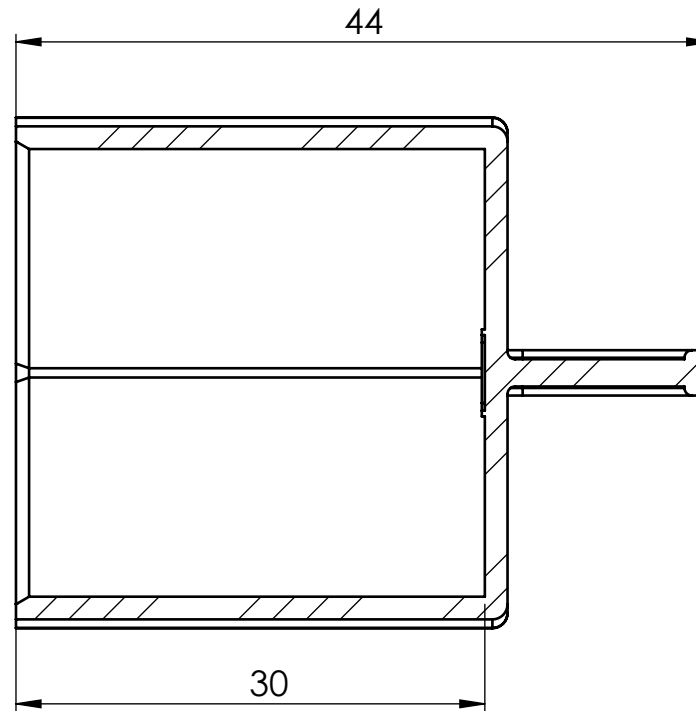
SECTION X-X
