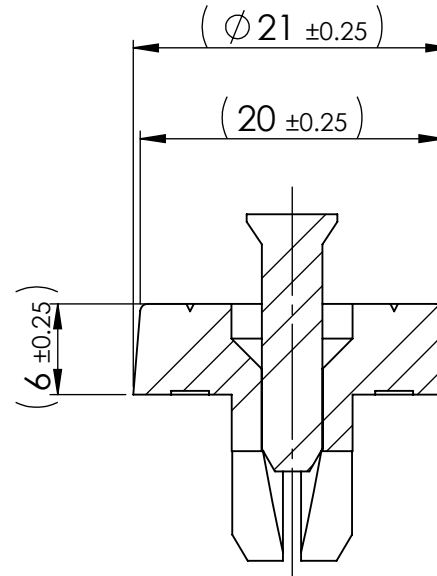
SECTION Y-Y
