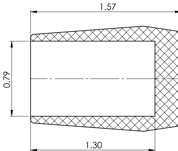
SECTION Y-Y
