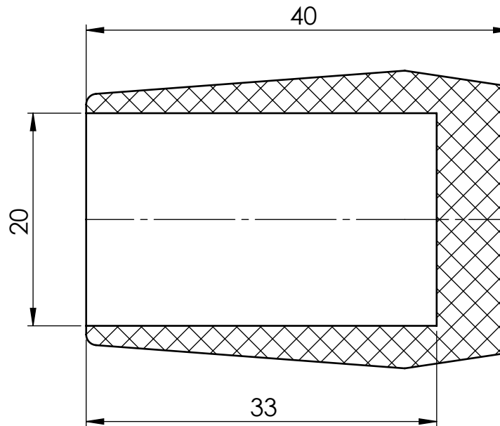
SECTION Y-Y
