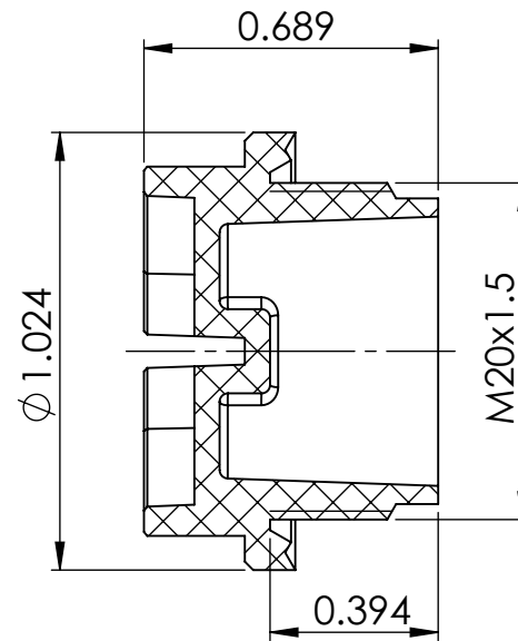
SECTION Y-Y
