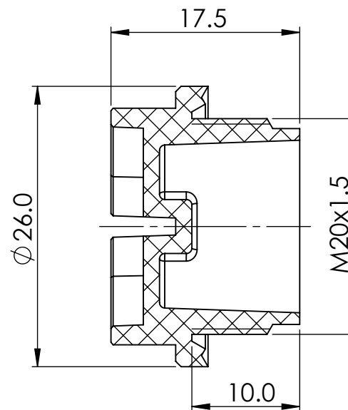
SECTION Y-Y
