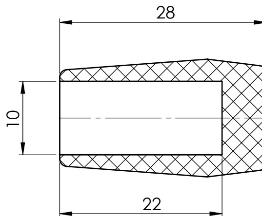
SECTION Y-Y
